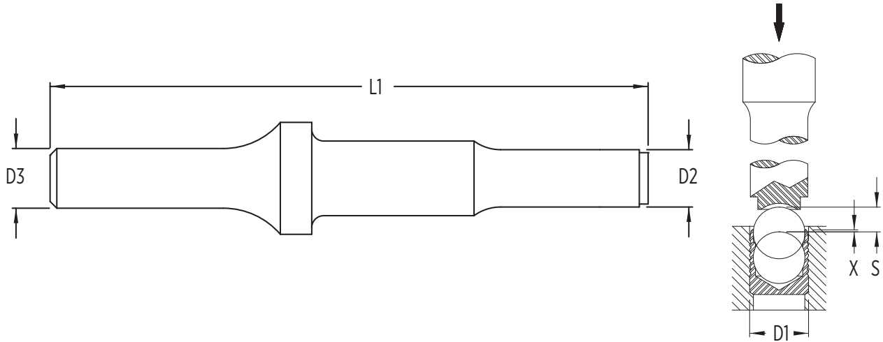
EIS-11, EIS-31 and EIS-33 (Dimensions in mm unless otherwise specified)
